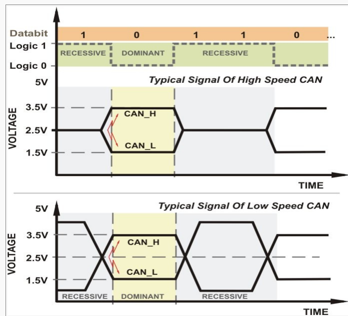
Figure 1: Typical signal of High & Low speed CAN.
